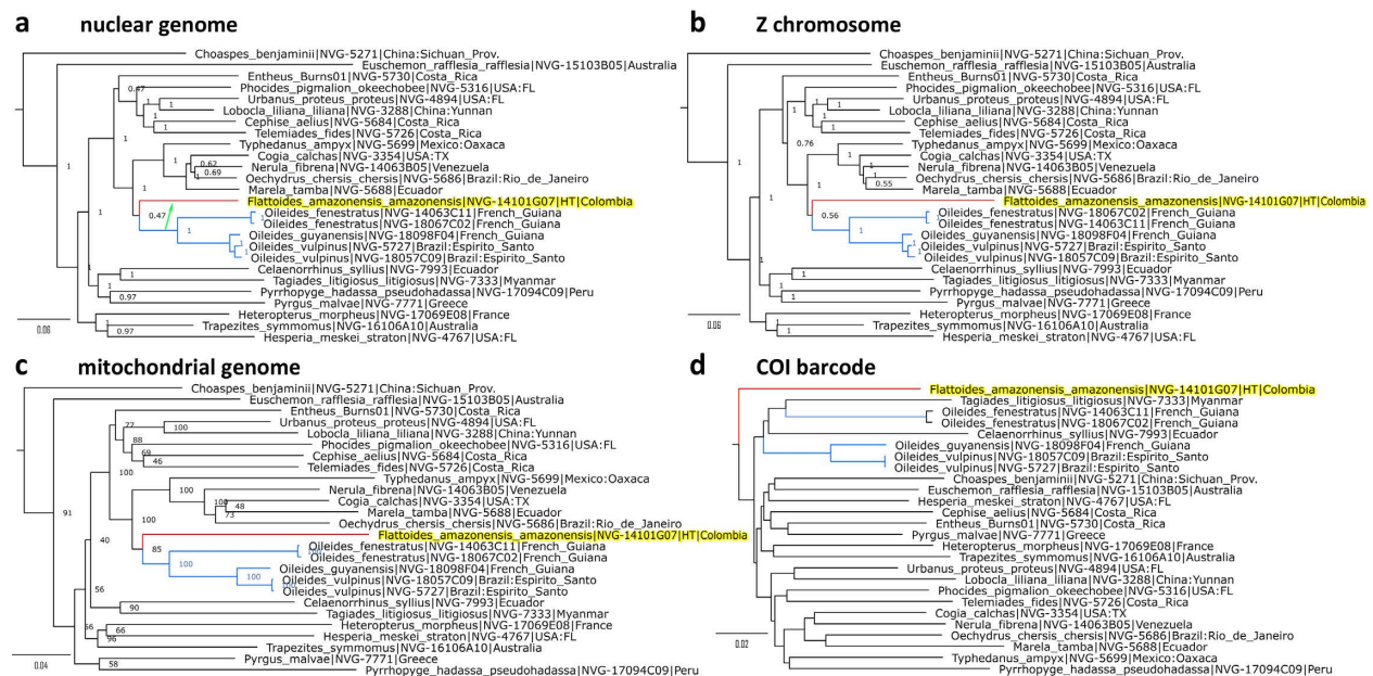
Figure 2. Genomic trees of Eudaminae and representatives of other Hesperidae subfamilies. The trees are built from protein-coding regions in different genomic partitions: a) Nuclear genome. b) Z chromosome. c) Mitochondrial genome; d) COI barcode. The trees are rooted with Pterourus glaucus (NVG-1670), not shown. See Table 1 and Table S1 in the Supplemental file deposited at https://osf.io/5cfht/?view_only=21eb53b6f8f344afae3de2be90bf5d2 for additional data about these specimens. Where possible, taxa are ordered similarly to that in the nuclear genome tree. Names of species placed in new genera described in this work are highlighted in yellow and clades of these genera are colored in red. Clades for genera where these species were placed previously are colored in blue and green arrow points from the former genus to the new genus (only on nuclear genome tree). Names of genera resurrected from synonymy are highlighted in cyan. Names of genera that form new genus-species combinations proposed in this work are highlighted in magenta. Statistical support values are shown by nodes in all but the COI barcode trees. COI barcode NJ dendrogram is given for comparison and is not expected to reflect phylogeny. The same notations are used in Fig. 2–13.
